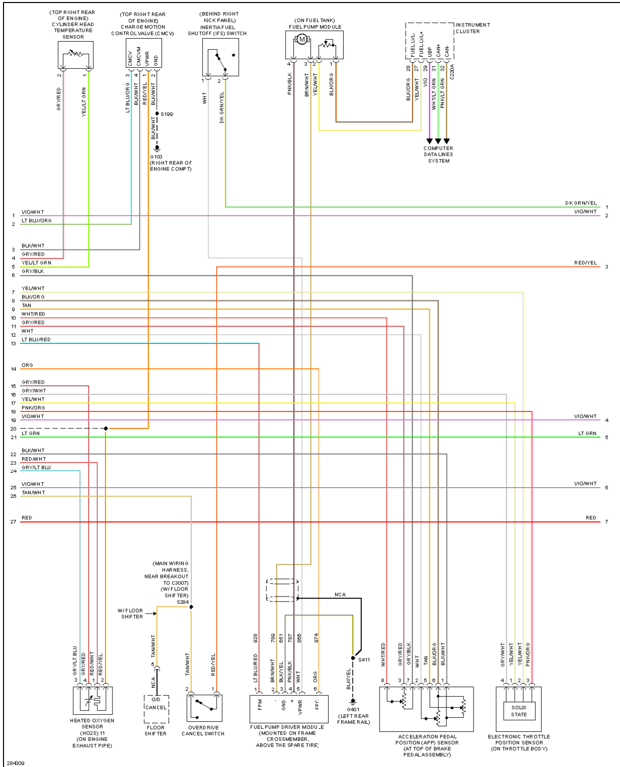
Fig. 29: 5.4L, Engine Performance Circuit (4 of 6)
