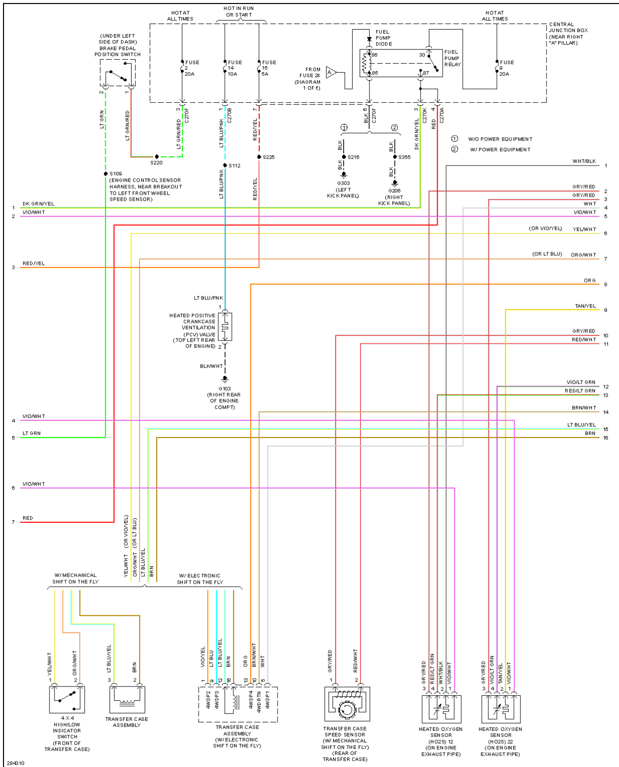
Fig. 30: 5.4L, Engine Performance Circuit (5 of 6)
