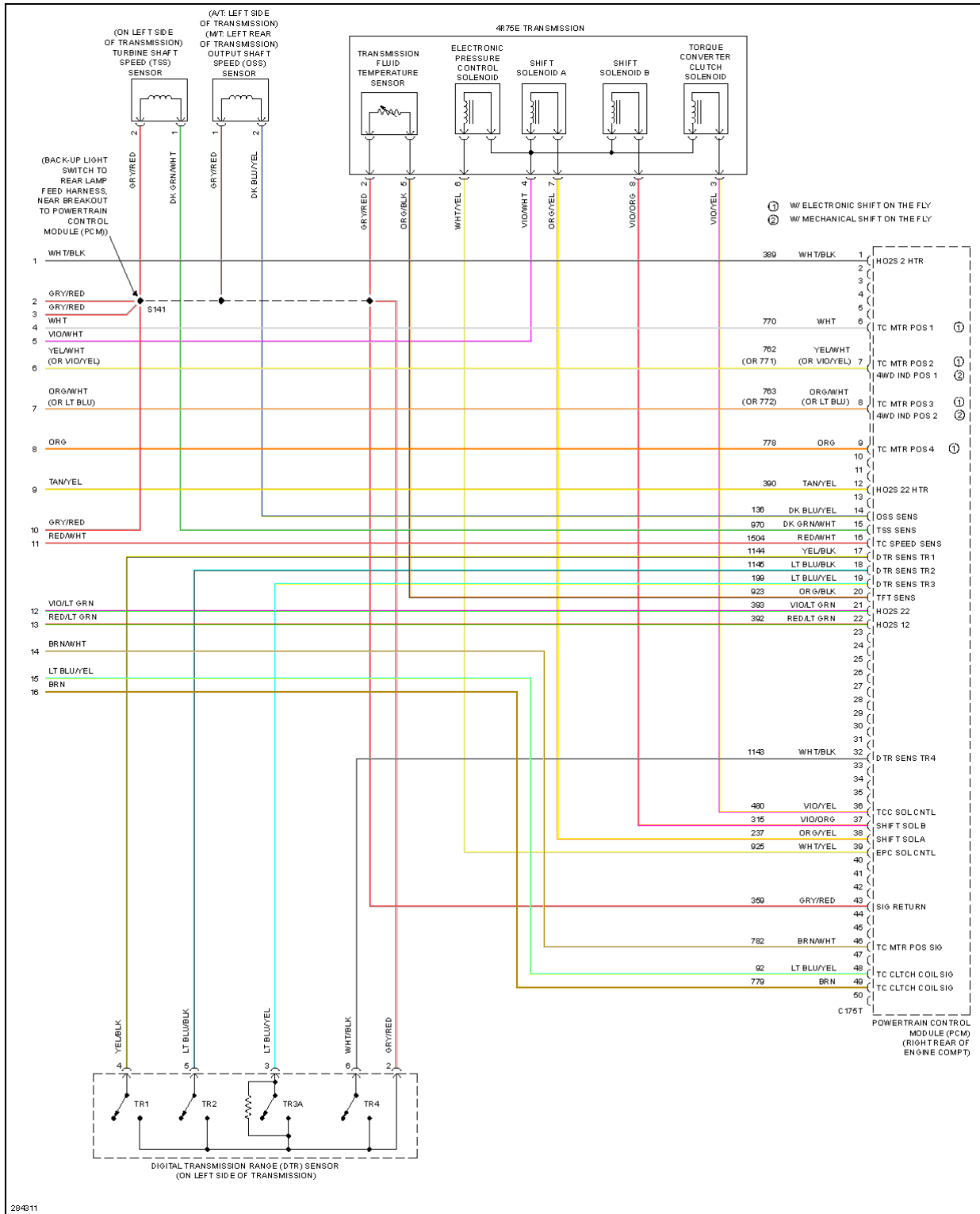
Fig. 31: 5.4L, Engine Performance Circuit (6 of 6)
