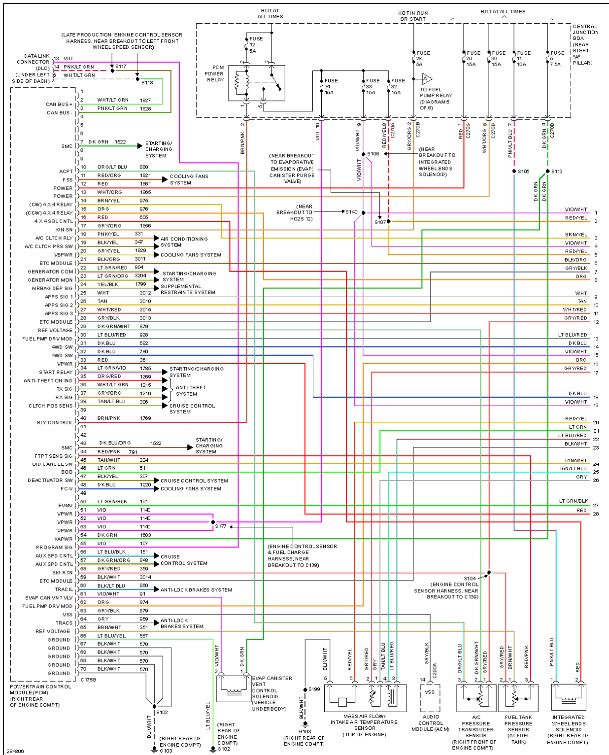
Fig. 26: 5.4L, Engine Performance Circuit (1 of 6)
